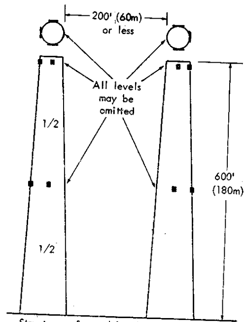
Structures of equal height. Number of levels depend upon height of structure. Lights on both structures to be synchronized. 17. f. (2)
