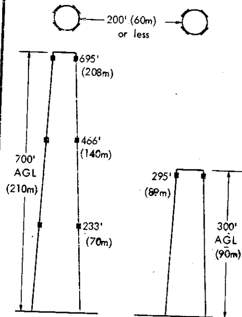
One structure higher than adjacent structure and light levels are not on same horizontal planes. 17. f. (2)
