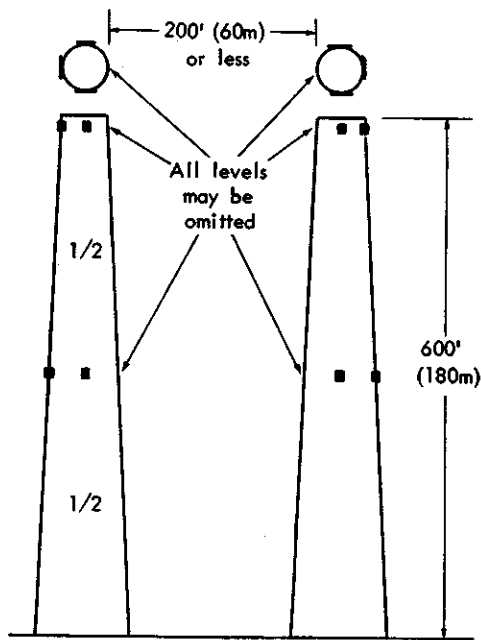
Structures of equal height. Number of levels depend upon height of structure. Lights on both structures to be synchronized.
