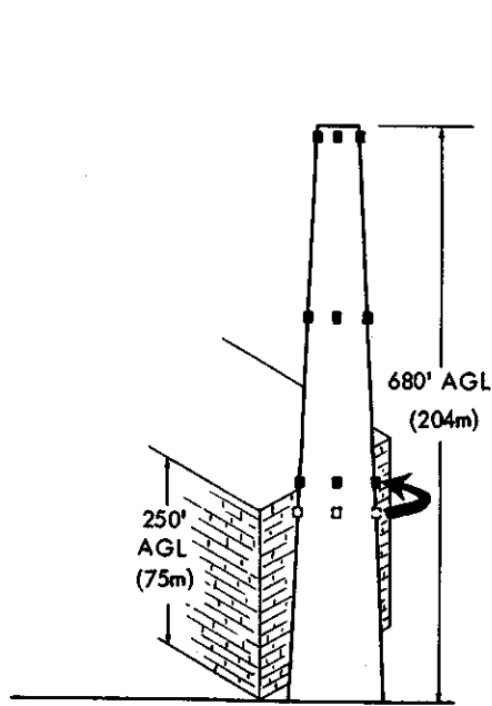
Lowest level should be above adjacent structure.
