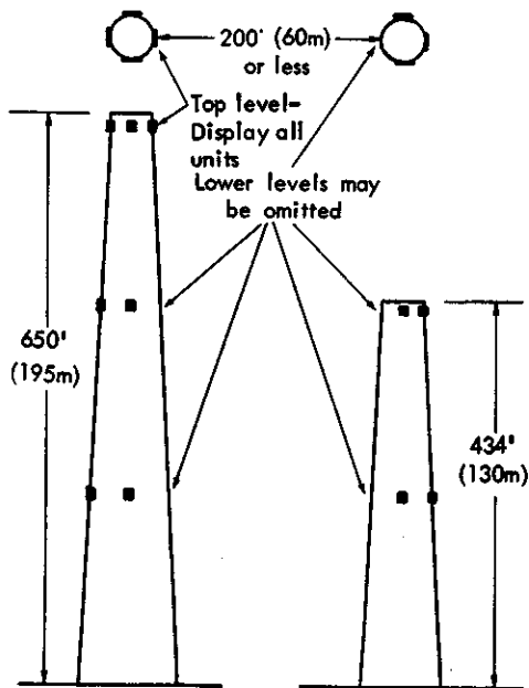
One structure higher than adjacent structure and light levels are on same horizontal plane. Lights on both structures to be synchronized.
