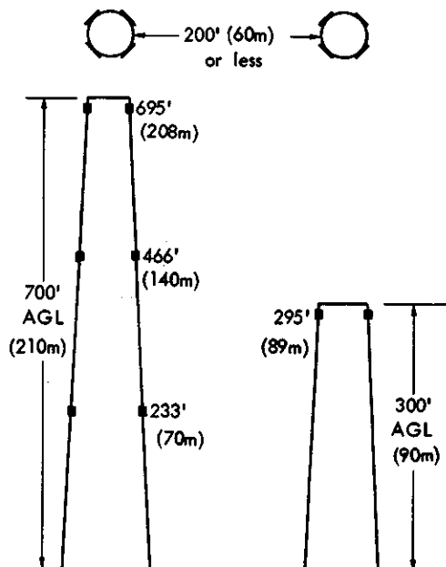
One structure higher than adjacent structure and light levels are not on same horizontal planes.
