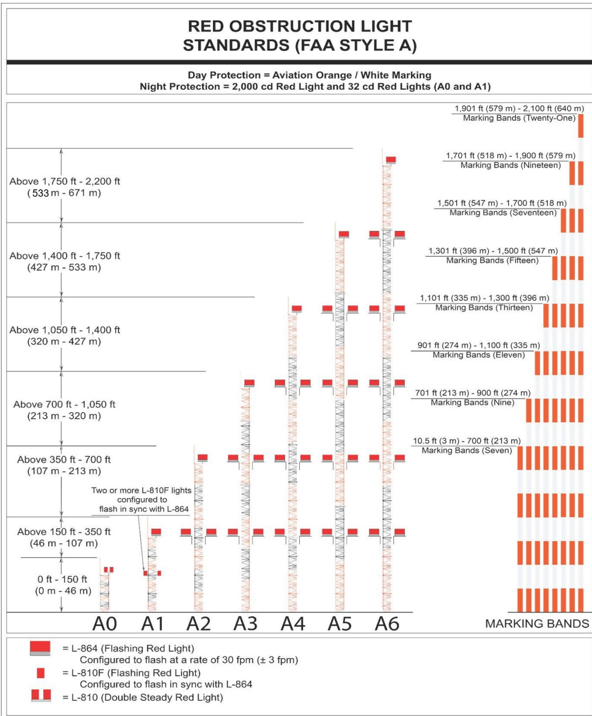
Figure A-6. Red Obstruction Light Standards (FAA Style A)
