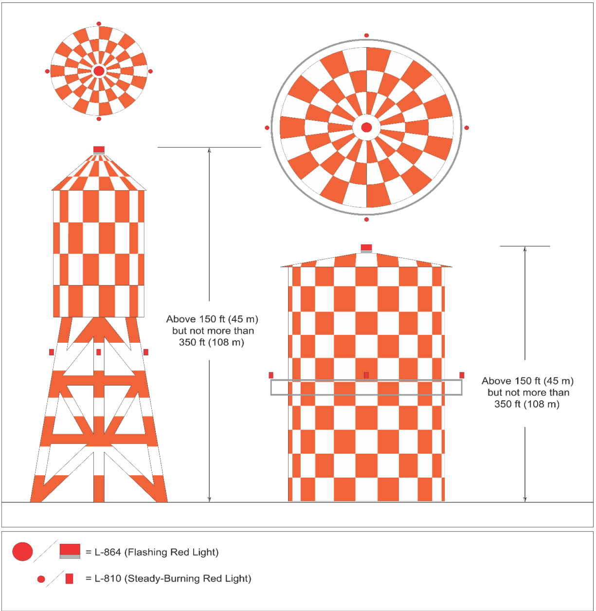
Figure A-3. Marking and Lighting of Water Towers, Storage Tanks, and Similar Structures
