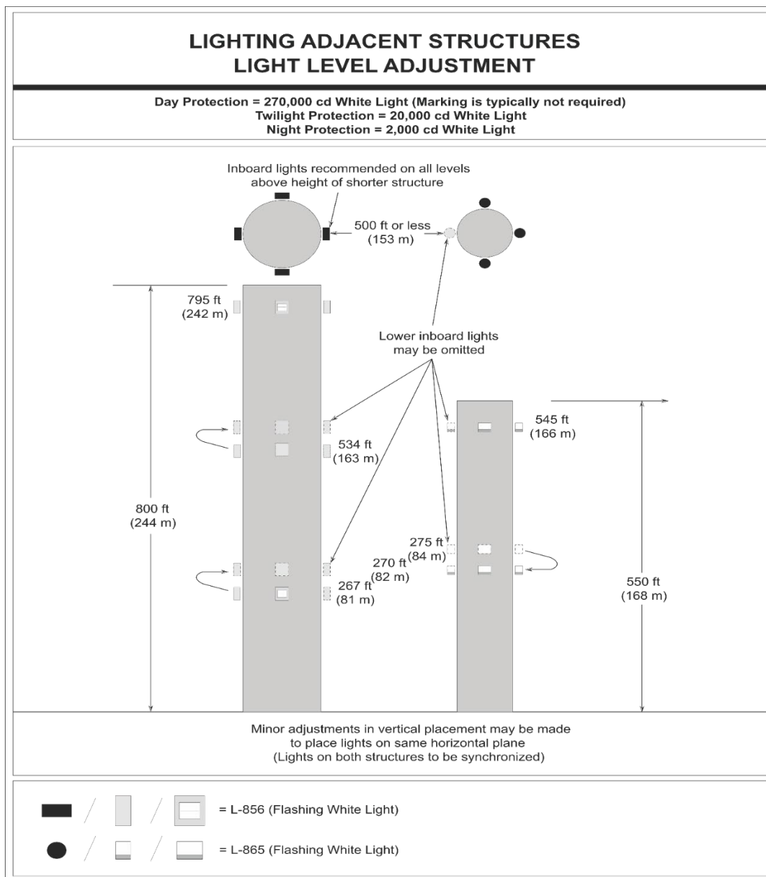
Figure A-11. Lighting Adjacent Structures—Light Level Adjustment
