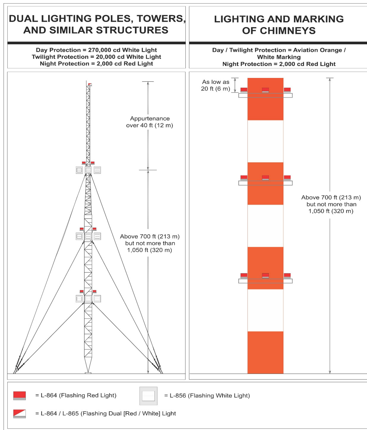
Figure A-7. Dual Lighting of Poles, Towers, and Similar Structures/Lighting and Painting of Chimneys
